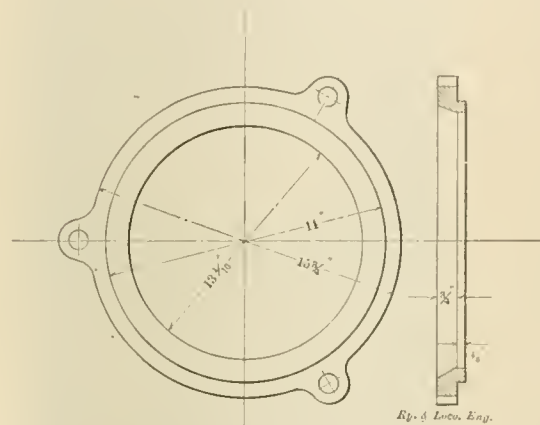
GUIDE FOR PUTTING PISTON VALVES IN PLACE.
